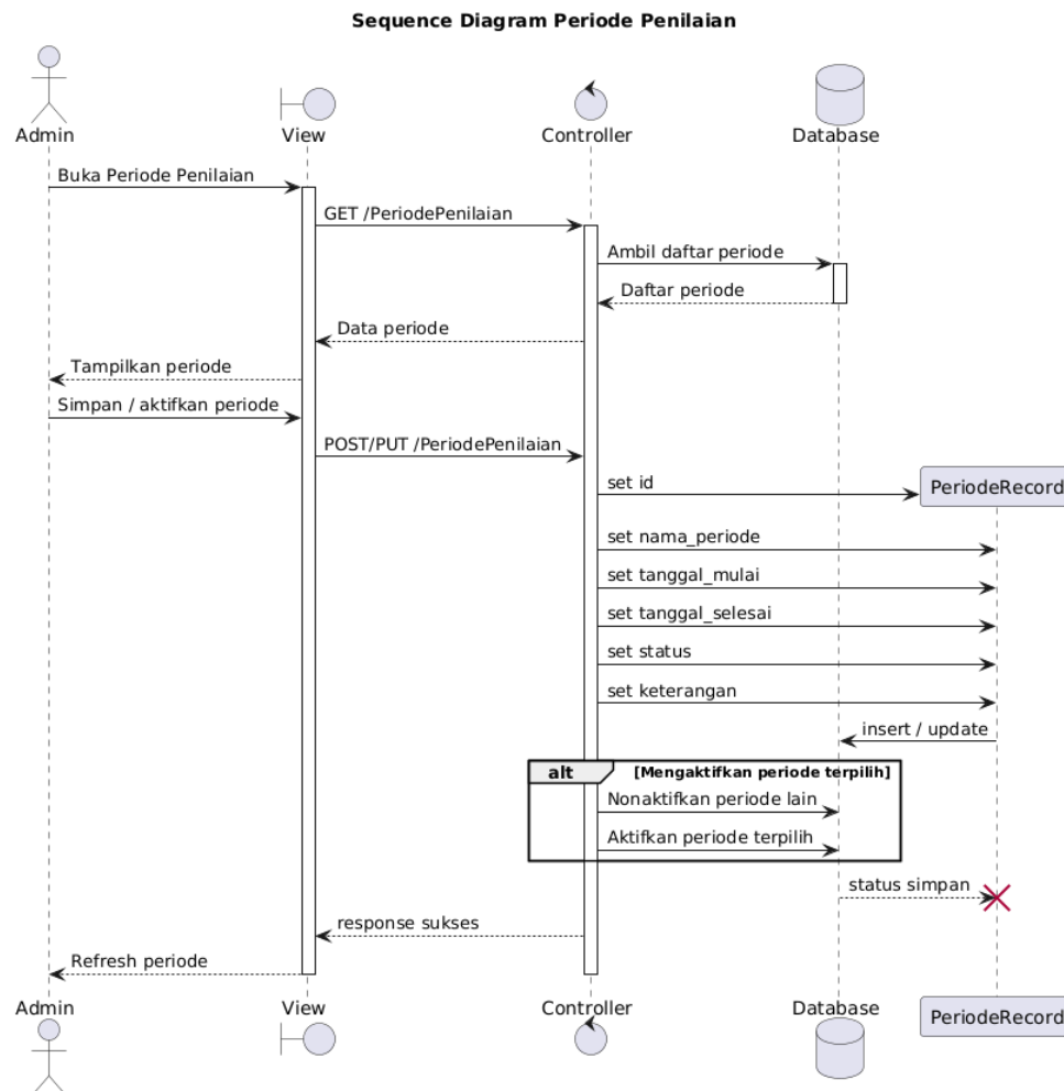
Gambar 4.26 Sequence Diagram Periode Penilaian Sumber : Hasil Rancangan
