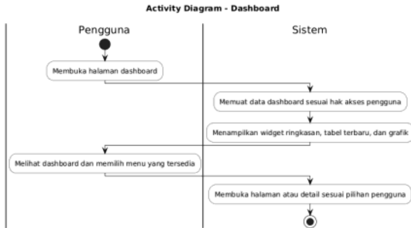
Gambar 4.7 Activity Diagram Dashboard Sumber : Hasil Rancangan
