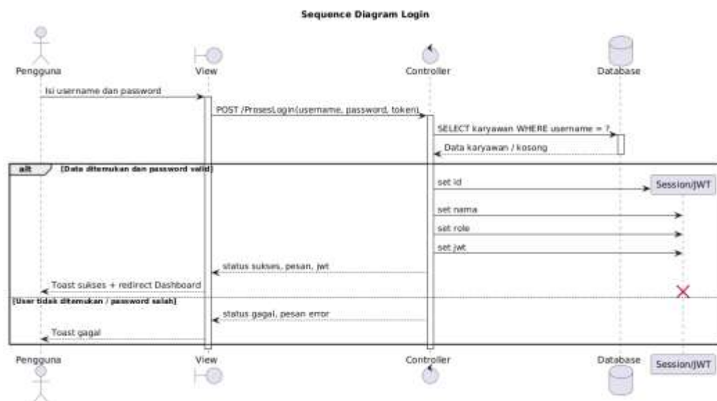
Gambar 4.20 Sequence Diagram Login
