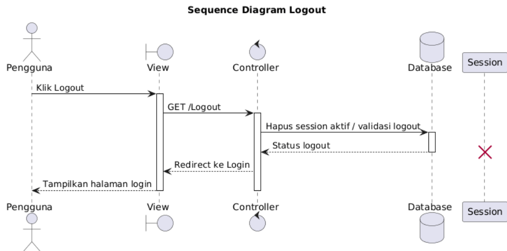
Gambar 4.21 Sequence Diagram Logout Sumber : Hasil Rancangan
