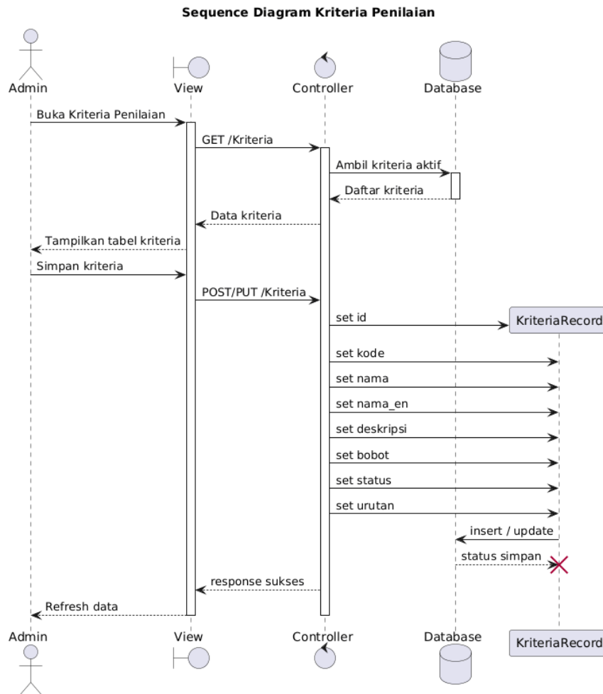
Gambar 4.25 Sequence Diagram Kriteria Penilaian Sumber : Hasil Rancangan
