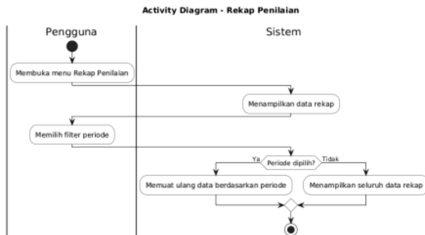
Gambar 4.12 Activity Diagram Rekap Penilaian
