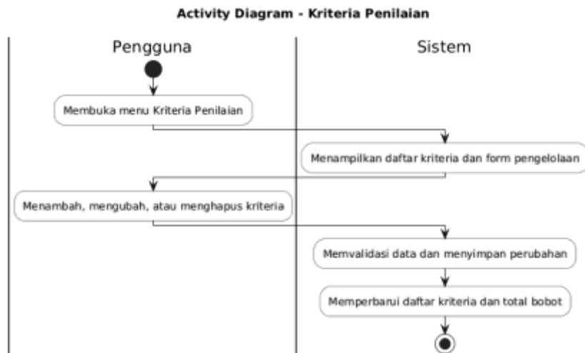
Gambar 4.10 Activity Diagram Kriteria Penilaian Sumber : Hasil Rancangan
