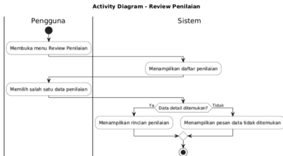
Gambar 4.15 Activity Diagram Review Penilaian Sumber : Hasil Rancangan
