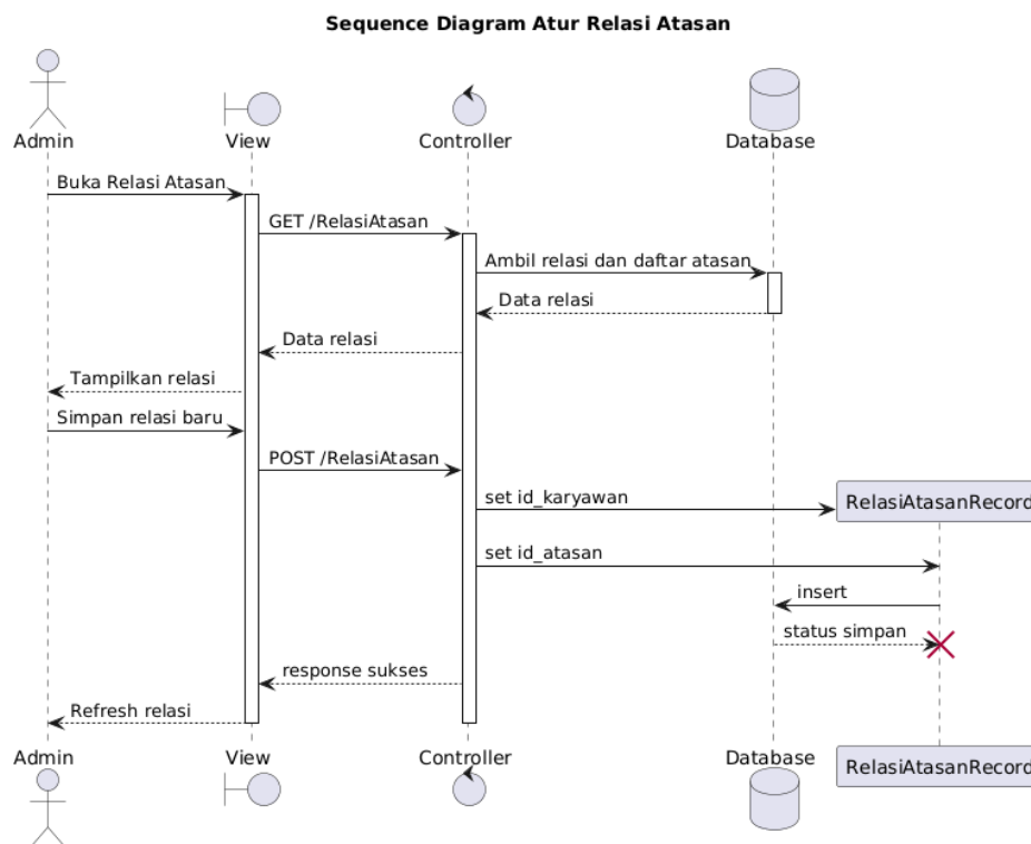
Gambar 4.24 Sequence Diagram Relasi Atasan
