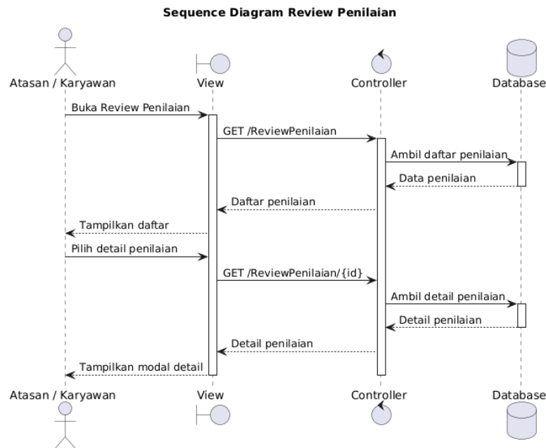
Gambar 4.30 Sequence Diagram Review Penilaian
