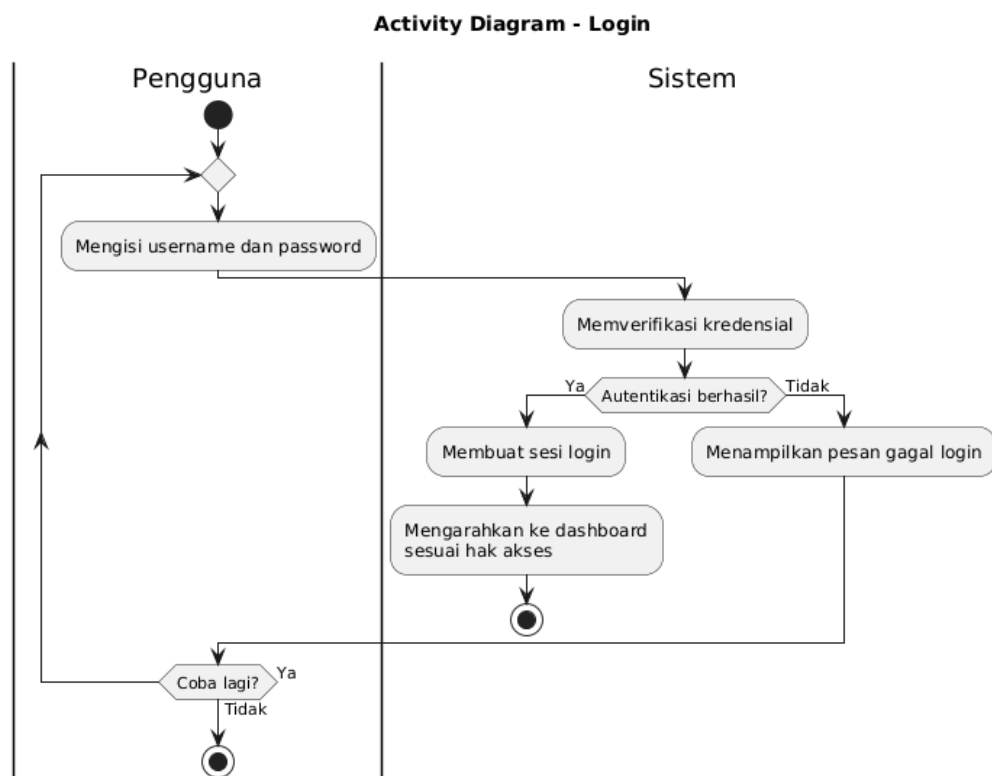
Gambar 4.5 Activity Diagram Login
