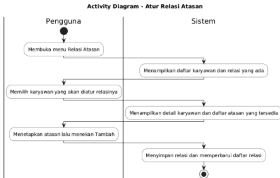
Gambar 4.9 Activity Diagram Atur Relasi Atasan Sumber : Hasil Rancangan
