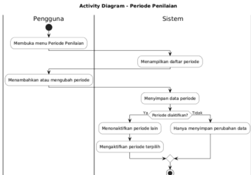
Gambar 4.11 Activity Diagram Periode Penilaian Sumber : Hasil Rancangan
