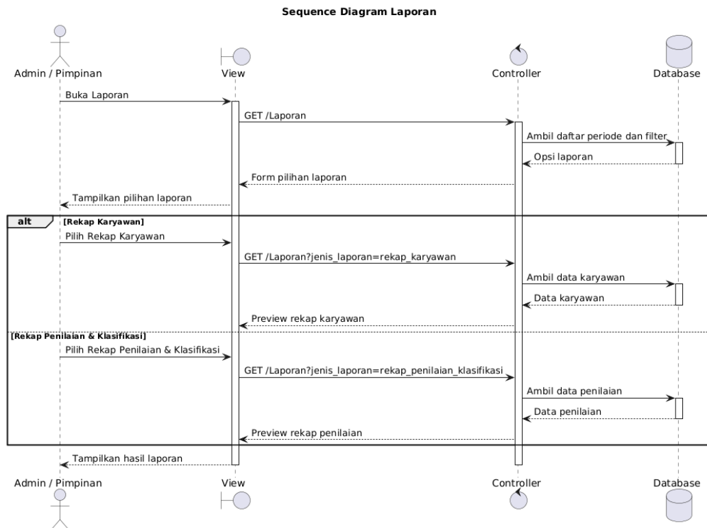
Gambar 4.32 Sequence Diagram Laporan
