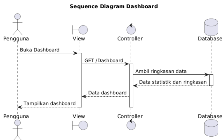
Gambar 4.22 Sequence Diagram Dashboard Sumber : Hasil Rancangan
